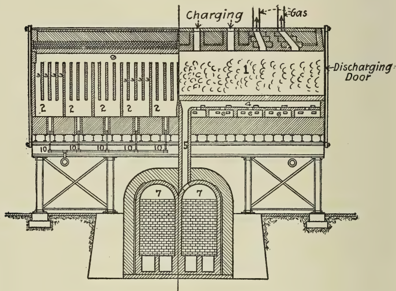
Fig. 90.—Otto-Hoffman Coke-oven.
